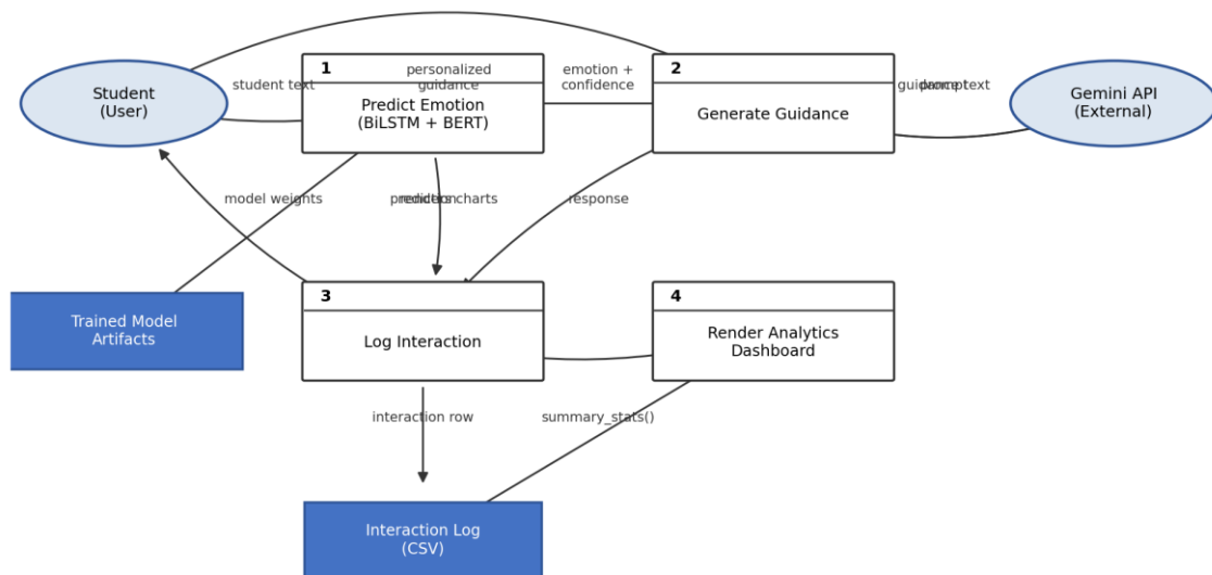
Data Flow Diagram — AI Learning Assistant
